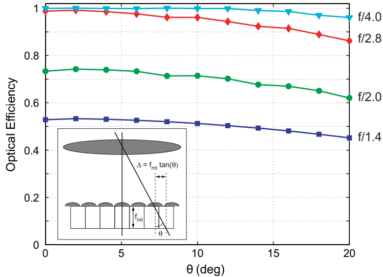
Figure 9. Light redirection. Simulations of light redirection for a 3- \mu m pixel with an 8- \mu m pixel height simulated for microlenses. The optical efficiency is measured as a function of the pixel location which is represented by angle of the chief ray in the material ( \theta ). The simulations offset the microlens from the pixel center by an amount \Delta computed as from the geometry shown in the inset. The curves measure efficiency for a series of diffraction-limited imaging lenses.
